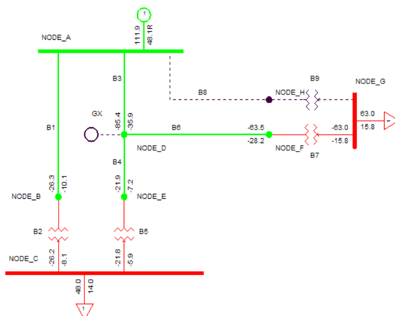
Figure 13 - Minimum Demand Scenario - Contingency Case 1.
