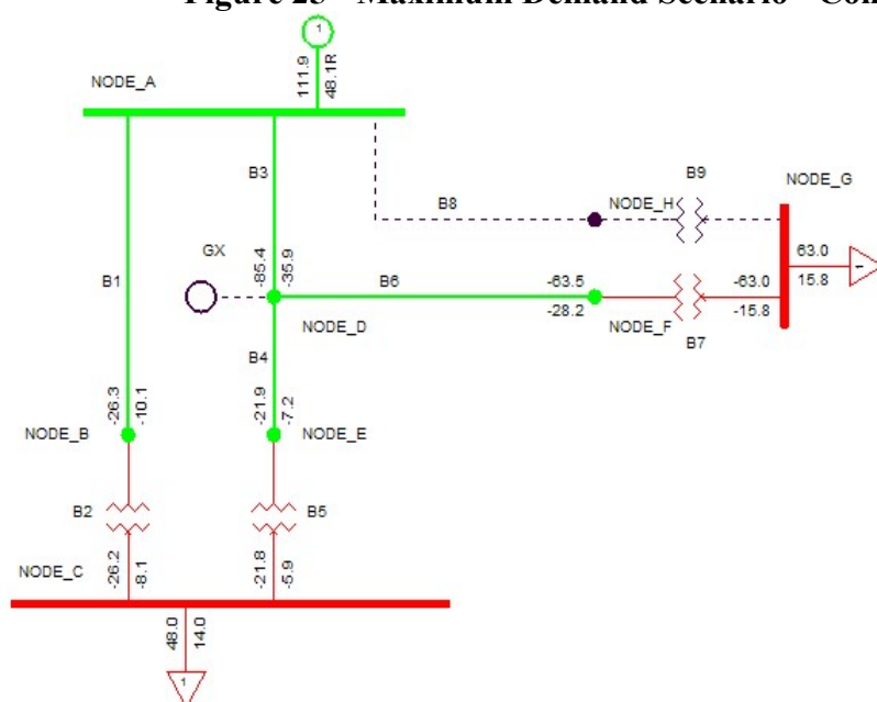
Figure 25 - Maximum Demand Scenario - Contingency Case 3.
