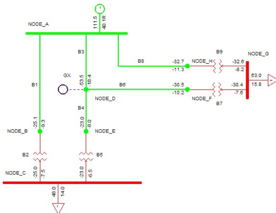
Figure 21 - Base Case Flows- Maximum Demand Scenario.
