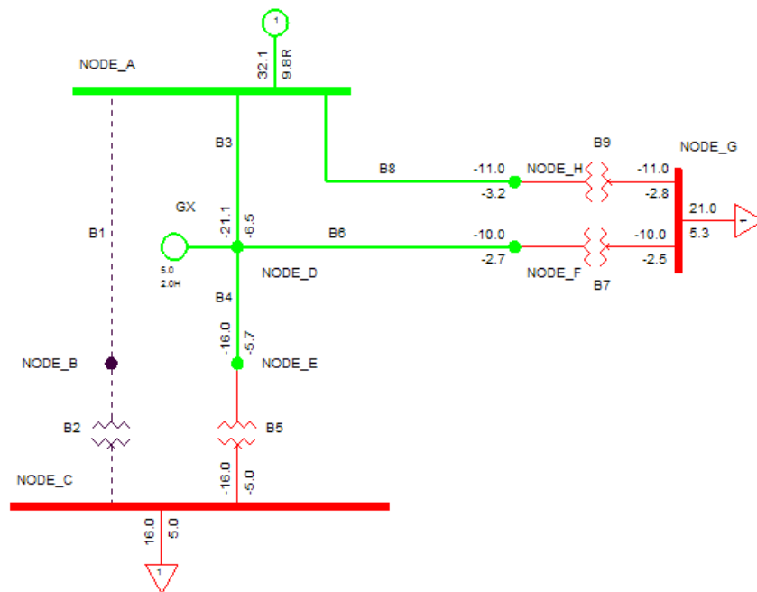
Figure 27 - Minimum Demand Scenario - Contingency Case 2
