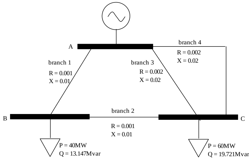
Figure 19 - Example network.
