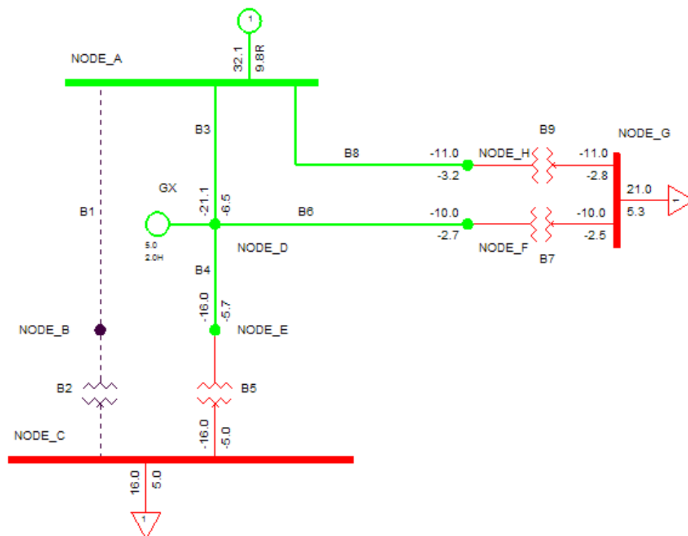
Figure 13 - Minimum Demand Scenario - Contingency Case 1.
