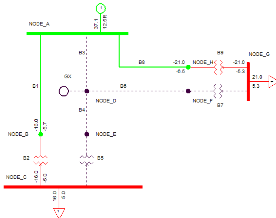
Figure 14 - Minimum Demand Scenario - Contingency Case 2
