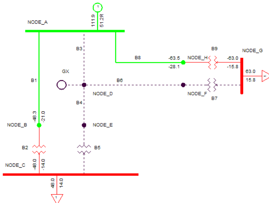
Figure 11 - Maximum Demand Scenario - Contingency Case 2.
