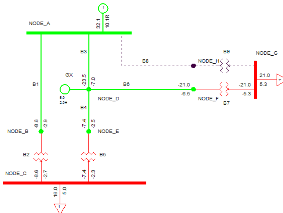
Figure 15 - Minimum Demand Scenario - Contingency Case 3.
