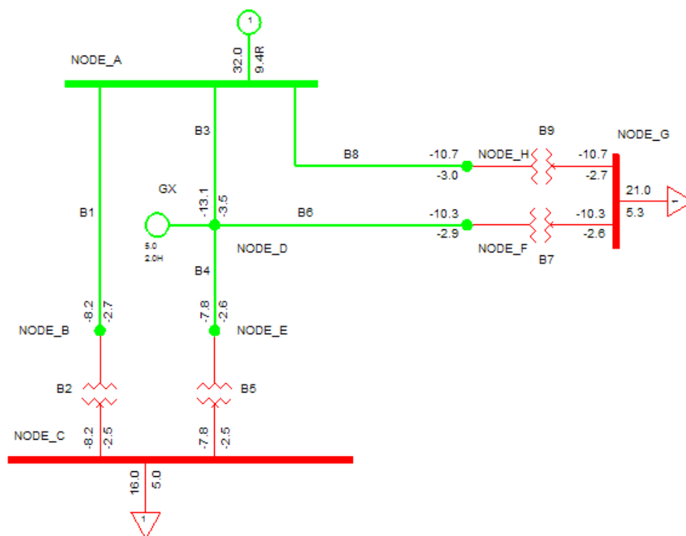
Figure 9 - Base Case Flows- Minimum Demand Scenario.
