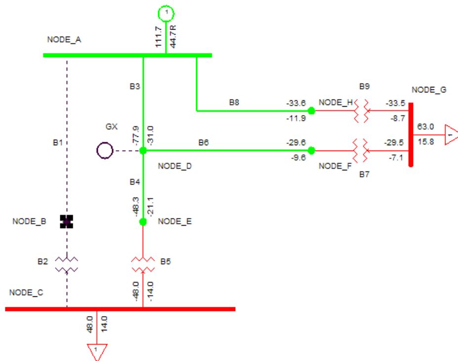
Figure 10 - Maximum Demand Scenario - Contingency Case 1.
